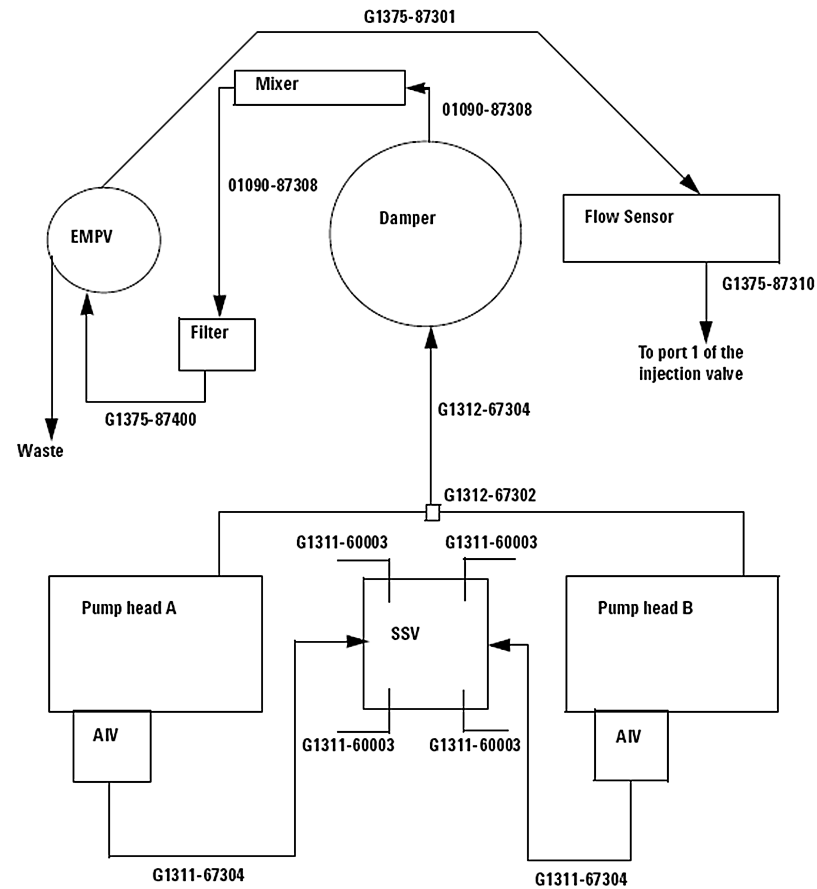
Pump flow connection
