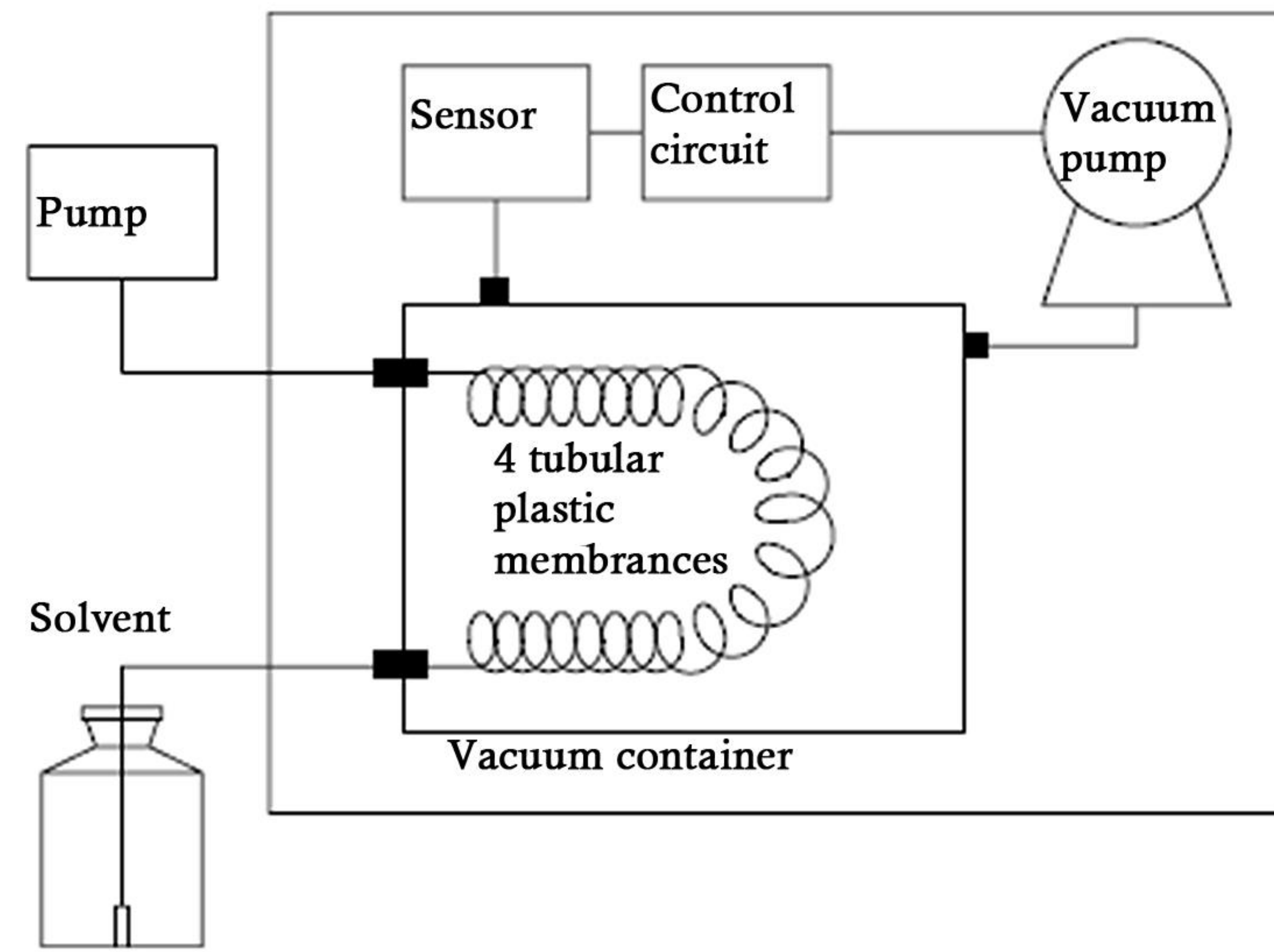
Vacuum degasser
