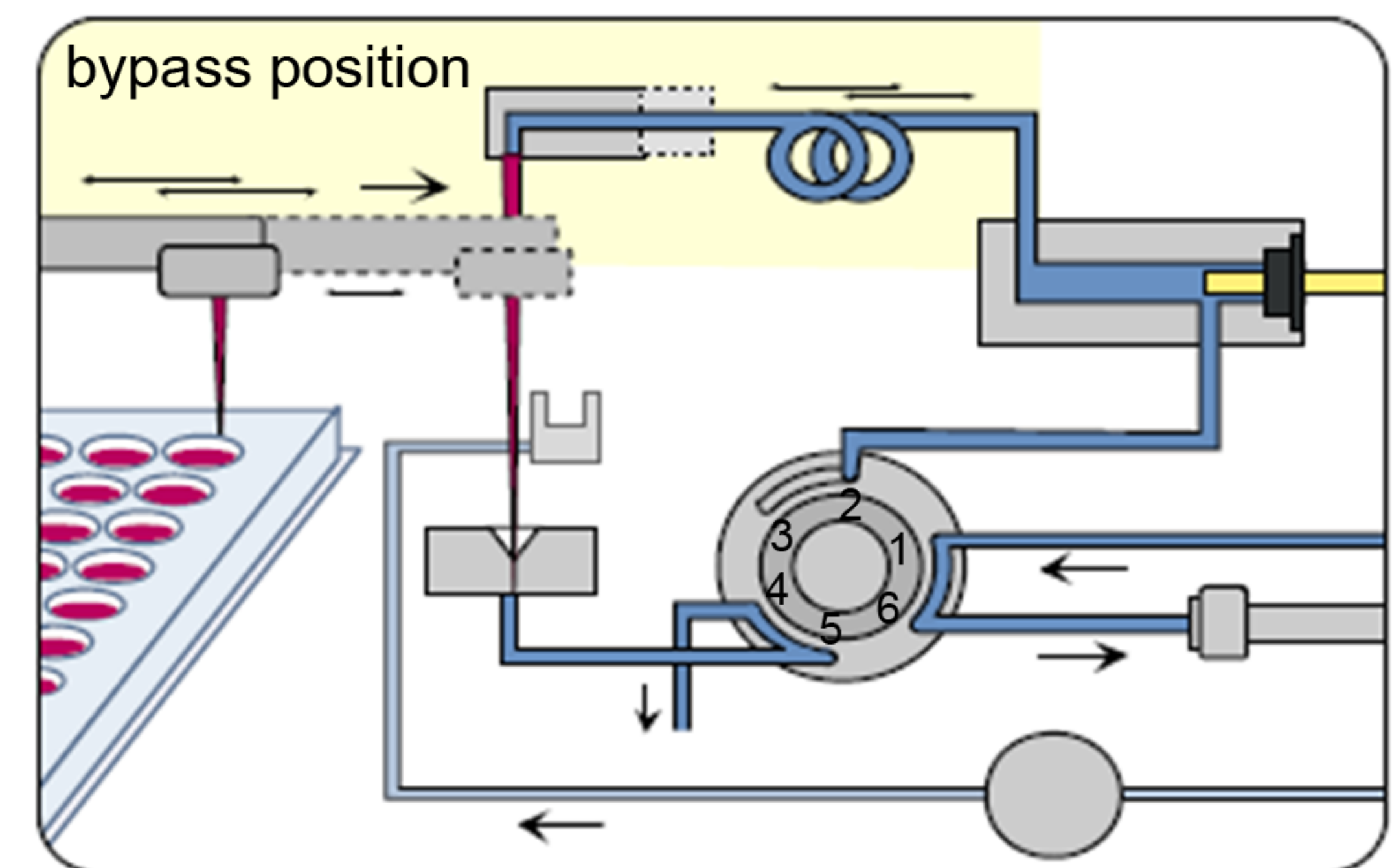
Autosampler injection sequence
